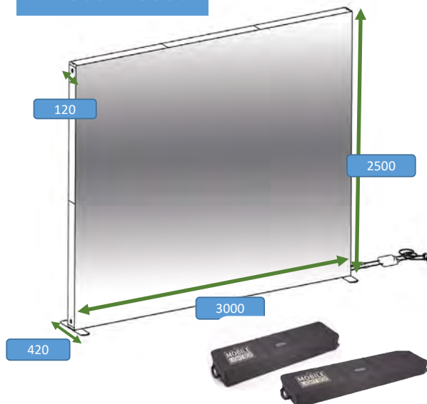
H2500xW3000
