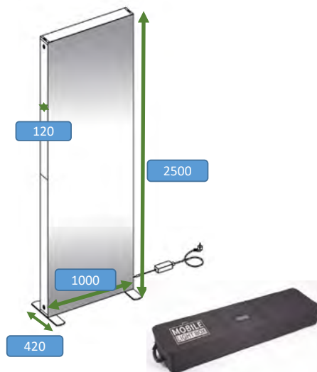
H2500xW1000
